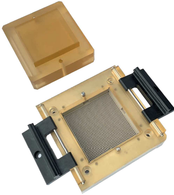
IC Socket for high pin count package
