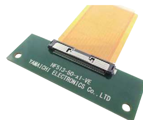
FPC/FFC Non-ZIF FPC/FFC Connector Non-ZIF Type 125°C Heat-resistant Type
