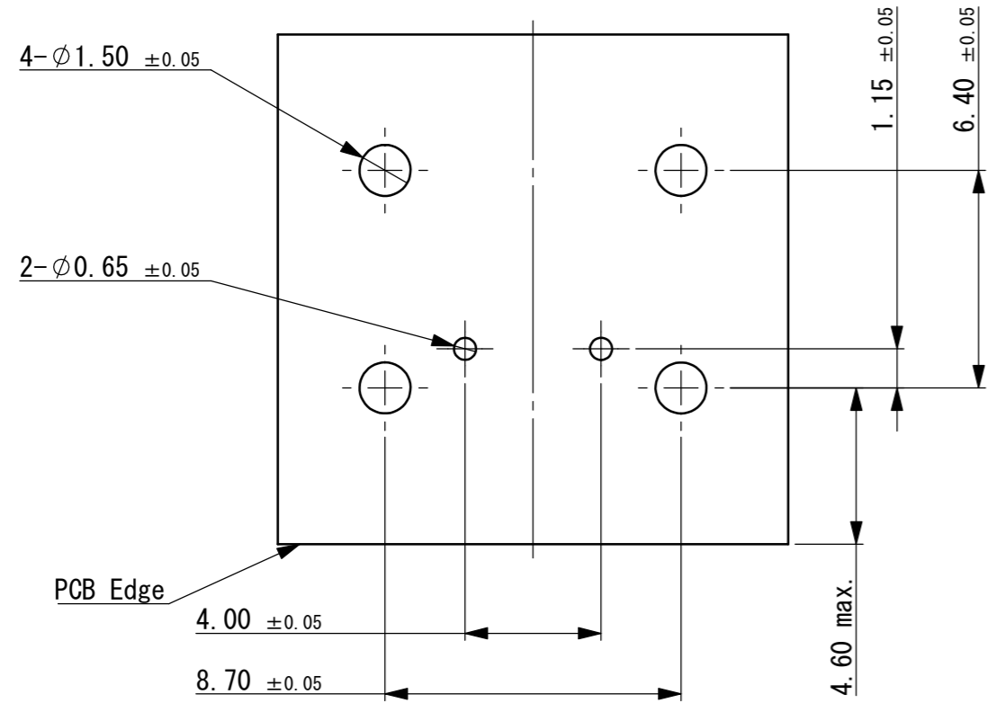
PCB Hole Pattern (FOR REFERENCE ONLY)
