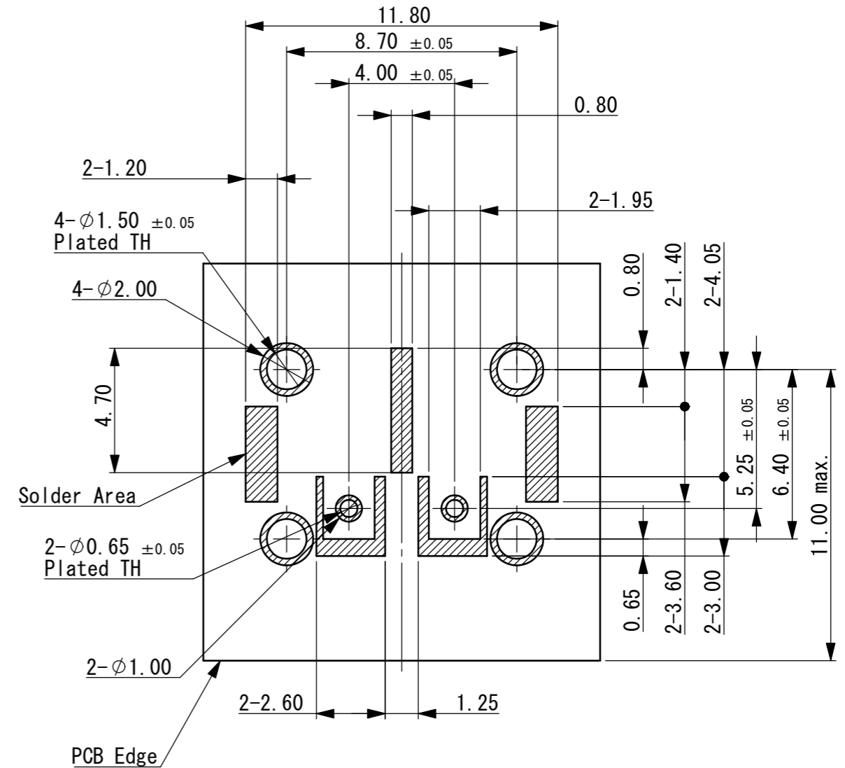
PCB Layout for Reflow Solder (FOR REFERENCE ONLY)
